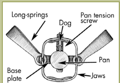
Figure MK8. Double-longspring trap with double-jaw
