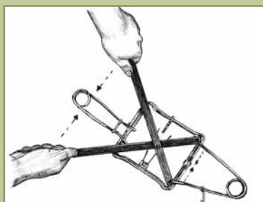
Figure MK3b. Using setting tool
