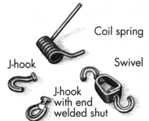
Figure 16. Trap components
