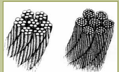
Figure 3a. 7 x 7 and 7 x 19 Cable strands
